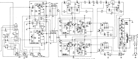
QUAD 33 Control Unit (Up to Serial No. 11503)
